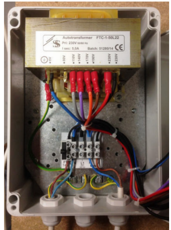
When wiring is complete controller should appear as above.
